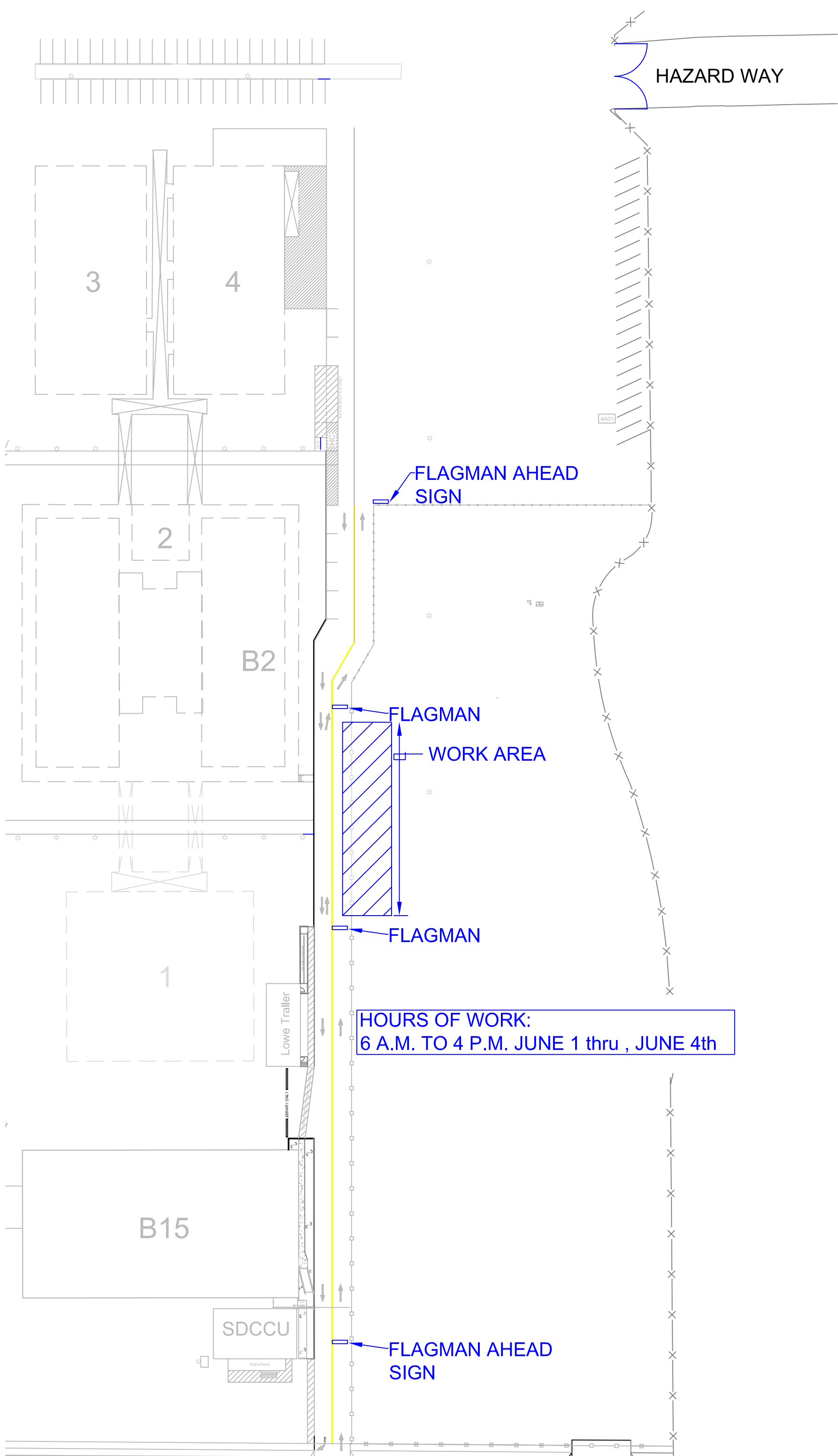
Site Utilization Plan for PS-A Joint Trench Completion Work Performed 6/1 thru 6/4/10
